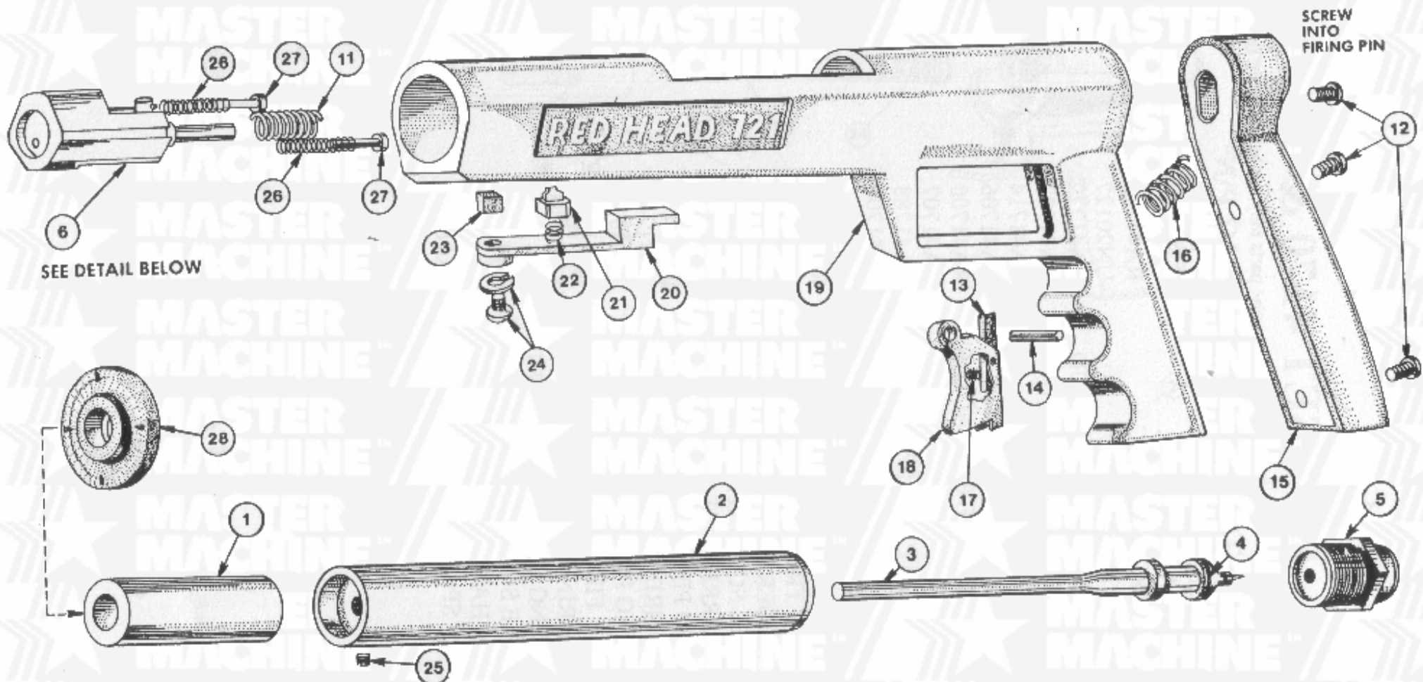
THE FIRING SYSTEM Detail Reversed For Clarity
